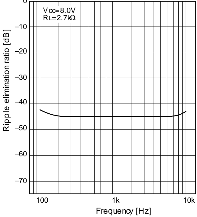
Ripple elimination ratio (PBOUT) Ta=25°C
